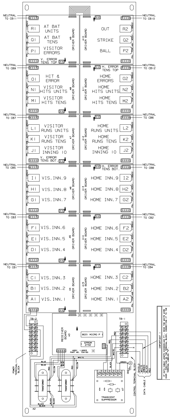
CONTROLLER ASSEMBLY
